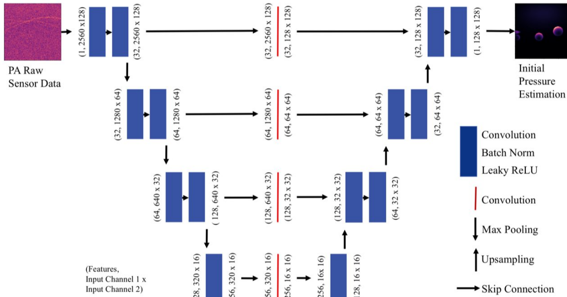
Figure 3. Architecture of the direct reconstruction U-Net. The modified U-Net is trained to estimate the initial pressure distribution directly from the PA raw sensor data. The skip connections of the U-Net include a convolutional layer that resizes the information to the target resolution. The contracting and expansive layers are the same as used with the standard U-Net.
