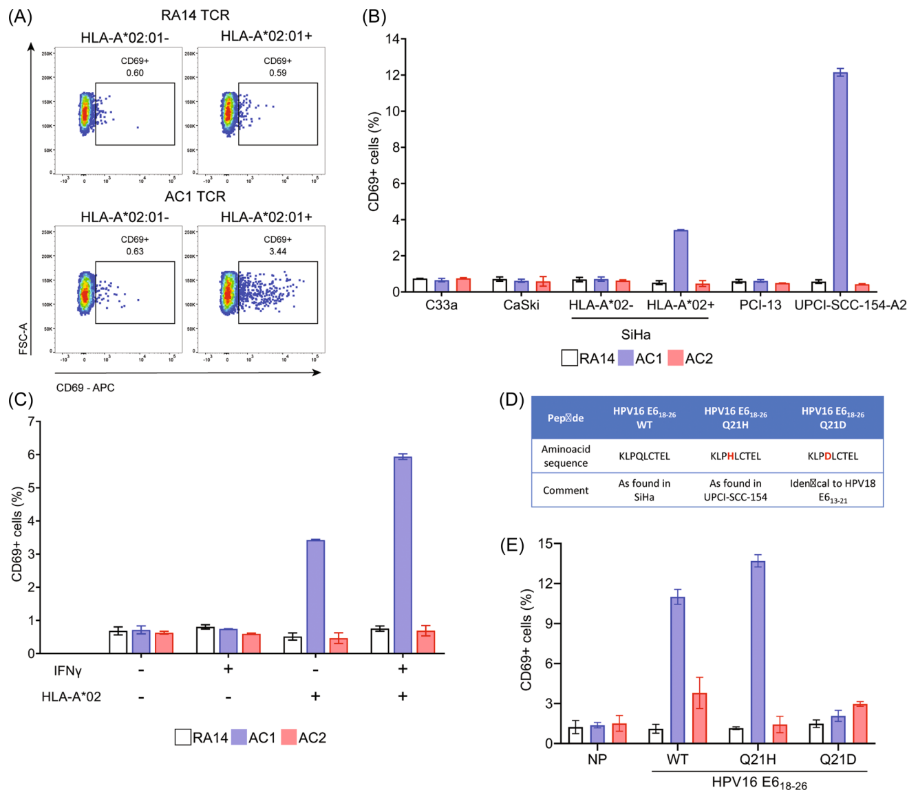
FIGURE 2 Activation of Jurkat J76/CD8 cells expressing AC1 or AC2 upon Coculture with HPV16 + cancer cell lines. Jurkat J76/CD8 cell lines stably expressing the AC1, AC2 or RA14 TCR were cocultured for 18 h with the indicated cancer cell lines. Then, the Jurkat cells were retrieved and stained with anti-murine TRBC-PECy7 and anti-CD69-APC. (A) flow cytometry graphs showing the gating of CD69 + Jurkat cells after co-incubation with SiHa cells HLA-A*02:01 + or HLA-A*02:01 - . (B) Histogram representing the frequencies of CD69 + Jurkat cells after co-incubation with the following cell lines: C33a (HPV16 - /HLA-A*02:01 + ), CaSki (HPV16 + /HLA-A*02:01 + ), SiHa (HPV16 + ), SiHa-A2 (HPV16 + /HLA-A*02:01 + ), PCI-13 (HPV16 - /HLA-A*02:01 + ), and UPCI-SCC-154-A2 (HPV16 + /HLA-A*02:01 + ). The percentage of CD69 + Jurkat cells after Coculture with the respective cancer cell lines is shown as mean \pm Standard deviation of three independent experiments. (C) SiHa/HLA-A*02:01 + cells were stimulated with IFN \gamma (50 ng/mL) for 24 h before starting co-cultures with the Jurkat J76/CD8 cells expressing the indicated TCRs. The percentages of CD69 + Jurkat cells after coculture in the presence or absence of IFN \gamma are shown as mean \pm Standard deviation of three independent experiments. (D) Two E6 peptide variants used for further functional tests: HPV16 E6 18-26 containing the Q21H mutation that resembles the epitope potentially presented by the UPCI-SCC-154-A2 (HLA-A*02:01 + ) cells; and E6 18-26 containing the Q21D mutation identical to the HPV18 E6 13-21 epitope, which is predicted to be presented by HPV18 + cells (E) Activation of Jurkat J76/CD8 cells stably expressing the indicated TCRs after Coculture with T2 cells preincubated with no peptide (NP) or with either E6 18-26 peptide variant (0.1 \mu M). After loading the T2 cells for 3 h, the cells were washed and cocultured with the Jurkat J76/CD8 cell lines for 18 h. Afterwards, the cells were retrieved and stained with anti-CD19-PE, anti-murine TRBC-PECy7 and anti-CD69-APC. T2 cells were excluded by gating murine-TRBC + /CD19 - . Results from three independent experiments are shown as the mean \pm standard deviation.
