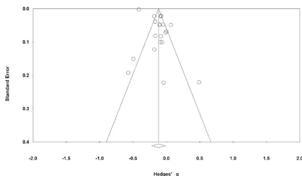
Fig. 3. Funnel plot of the meta-analysis.
