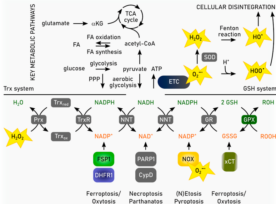
Fig. 2. Deregulated redox metabolome drives regulated necrosis. The two key thiol-dependent antioxidant systems in mammalian cells, the thioredoxin (Trx) and the glutathione (GSH) redox cycles are dependent on the presence of NAD(P)H cofactor that is restored by nicotinamide nucleotide transhydrogenase (NNT) within the mitochondria. Trx reductase (TrxR) utilizes NADPH to reduce Trx and other low molecular weight compounds. Peroxiredoxins (Prxs), on the other hand, accept electrons from Trx and subsequently scavenges hydrogen peroxide ( H_2O_2 ) and other organic hydroperoxides. Like TrxR glutathione reductase (GSR) uses electrons from NADPH to restore reduced GSH from its oxidized state (GSSG). GSH in turn is the main substrate of glutathione peroxidases (GPXs). Members of the GPX protein family convert hydrogen peroxide and lipid hydroperoxides into water and alcohols, respectively. Different redox couples are affected by different types of regulated necrosis. Ac-CoA: Acetyl-CoA, \alpha KG: \alpha -ketoglutarate, DHFR1: dihydrofolate reductase 1, FA: fatty acid, NAD: nicotinamide adenine dinucleotide, NADPH: nicotinamide adenine dinucleotide phosphate, Prx: peroxiredoxin, SOD: superoxide dismutase.
