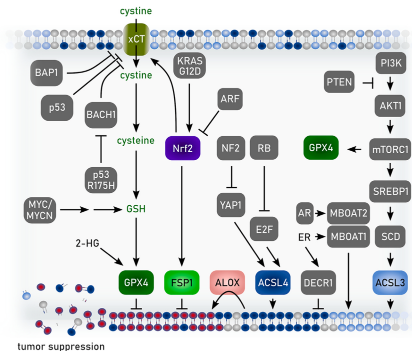
Fig. 15. Schematic overview of the complexity of different pathways modulating ferroptosis in cancer cells. p53 and BAP1 suppress SLC7A11 to restrain the uptake of cystine. NRF2 and MYC/MYCIN inhibit ferroptosis in both GPX4- or FSP1-dependent manner. KRAS G12D and ARF positively or negatively modulate NRF2 activities, respectively. NF2-YAP1 and RB-E2F axis regulate cell ferroptosis vulnerability by modulating ACSL4 expression and PUFA-PL content. Conversely, AR-MBOAT2, ER-MBOAT1, or PI3K-AKT-mTORC1-SREBP1-SCD pathways decrease cell sensitivity to ferroptosis by modulating MUFA-PL content. ACSL: acyl-CoA synthetase long-chain family member, AKT1: AKT serine/threonine kinase 1, ALOX: lipoxygenase, AR: androgen receptor, ARF: Tumor suppressor ARF, BAP1: BRCA1 associated protein 1, BACH1: BTB domain and CNC homolog 1, DEC1: 2,4-dienoyl-CoA reductase 1, E2F: E2F transcription factor 1, ER: estrogen receptor, FSP1: ferroptosis suppressor protein 1, GPX4: glutathione peroxidase 4, 2-HG: 2-hydroxyglutarate, KRAS: KRAS proto-oncogene, GTPase, MBOAT: O-acyltransferase domain containing, mTORC1: mammalian target of rapamycin complex 1, MYC: MYC proto-oncogene, MYCN: MYCN proto-oncogene, NF2: neurofibromin 2, NRF2: nuclear factor erythroid 2-related factor 2; PI3K: phosphatidylinositol 3-kinase; PTEN: phosphatase and tensin homolog, RB: RB transcriptional corepressor 1, SCD: stearoyl-CoA desaturase, SREBP1: sterol regulatory element-binding protein 1, xCT: SLC7A11 - solute carrier family 7 member 11, YAP1: Yes1 associated transcriptional regulator.
