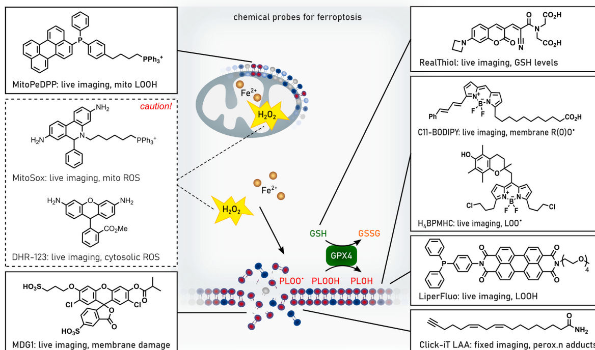
Fig. 19. Chemical probes for detecting ferroptosis. These probes can report on phospholipid peroxidation (C11-BODIPY, H 2 BPMHC, LiperFluo; including in mitochondria via MitoPeDPP); loss of plasma membrane integrity (MDG1); and depletion of antioxidant defenses e.g. GSH levels (RealThiol). Fluorescent “dihydro” probes claimed to report ROS levels (MitoSox, DHR-123) should only be used with caution.
