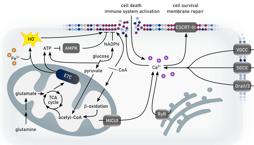
Fig. 9. Calcium signaling and energy metabolism in ferroptosis. Increased cytosolic calcium is one of the hallmarks of ferroptosis. It remains unclear, however, whether calcium ions enter the cell through membrane nanopores, through endogenous channels at the plasma membrane, or whether the ER or mitochondria are responsible for calcium transport, or a combination of those. Cytosolic calcium contributes to ferroptosis and to the subsequent release of intracellular components. Yet, calcium signaling also connects plasma membrane damage with the activation of membrane repair mechanisms that counterbalance cell death. Energetic metabolism centered around mitochondrial activity is the major source for the generation of free radicals and reactive oxygen species in the cell. Therefore, energetic metabolism plays a central role in ferroptosis induction. Related processes, such as glutamine anaplerosis, TCA cycle and electron transfer chain (ETC) activity, have all been demonstrated to be involved in ferroptosis. AMPK: AMP-activated protein kinase, ESCRTIII: endosomal sorting complex required for transport III, MICU1: Mitochondrial calcium uptake 1, ORAI: calcium channel protein, RyR: ryanodine receptor, SOCE: store-operated calcium entry, VGCC: voltage-gated calcium channels.
