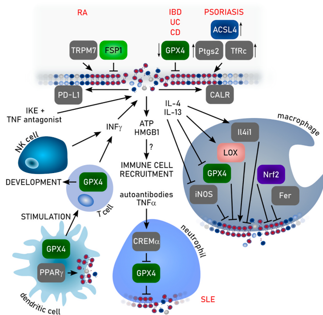
Fig. 12. Ferroptosis and immunity. Ferroptosis is induced in diseases such as rheumatoid arthritis (RA) via transient receptor potential cation channel, sub-family M, member 7 (TRPM7) and ferroptosis suppressor protein (FSP1), inflammatory bowel disease (IBD), ulcerative colitis (UC), Crohn's disease (CD) via decreasing glutathione peroxidase 4 (GPX4), and psoriasis via fatty acid-CoA ligase 4 (ACSL4), prostaglandin-endoperoxide synthase 2 (Ptgs2) and transferrin receptor (TfRc). Thereby, ferroptosis leads to exposure of programmed cell death ligand-1 (PD-L1) and calreticulin (CALR) as well as release of ATP and high mobility group box 1 (HMGB1) which facilitate immune cell recruitment. As potential therapeutic inducers of ferroptosis IKE in combination with TNF antagonists are discussed. In addition, interferon (INF) \gamma released by natural killer NK cells and T cells, which relay on GPX4 during development, contributes to ferroptosis induction. Ferroptosis is mediated in dendritic cells by peroxisome proliferator-activated receptor (PPAR) \gamma . During systemic lupus erythematosus (SLE) ferroptosis is facilitated by autoantibodies and TNF \alpha which induce cAMP-responsive element modulator (CREM) \alpha , a transcriptional repressor for GPX4, in neutrophils. In macrophages interleukin (IL) -4 and -13 contributes to ferroptosis by inducing lipoxygenases (LOX) and blocking GPX4 and inducible nitric oxide synthase (iNOS). Nevertheless, it inhibits ferroptosis via L-amino acid oxidase IL-4 induced gene-1 (IL4iL). Further, nuclear factor erythroid-2-related factor 2 (NRF2) and ferritin (Fer) protect macrophages from ferroptosis.
