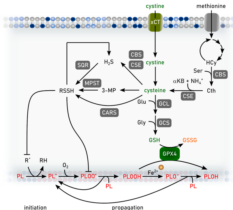
Fig. 7. Cysteine metabolism and ferroptosis. Schematic overview of the main pathways involved in cysteine uptake, de novo cysteine synthesis, and cysteine utilization that regulate ferroptosis sensitivity in cells. Cysteine can be taken up in its oxidized form cystine via the xCT transporter, or synthesized de novo from methionine and serine via the transsulfuration enzymes cystathionine \beta -synthase (CBS) and cystathionine \gamma -lyase (CSE). Production of glutathione (GSH) from cysteine supports the activity of glutathione peroxidase 4 (GPX4) to detoxify phospholipid hydroperoxides (PLOOH) and mitigate the propagation of the lipid peroxidation cycle. Moreover, cysteine-derived sulfane sulfur species (hydropersulfides, RSSH) act as radical trapping agents that can suppress the initiation and propagation of the radical chain reaction driving lipid peroxidation.
