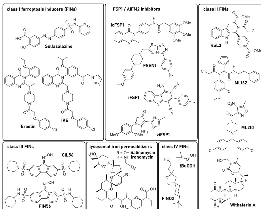
Fig. 13. Chemical structures of ferroptosis inducers.
