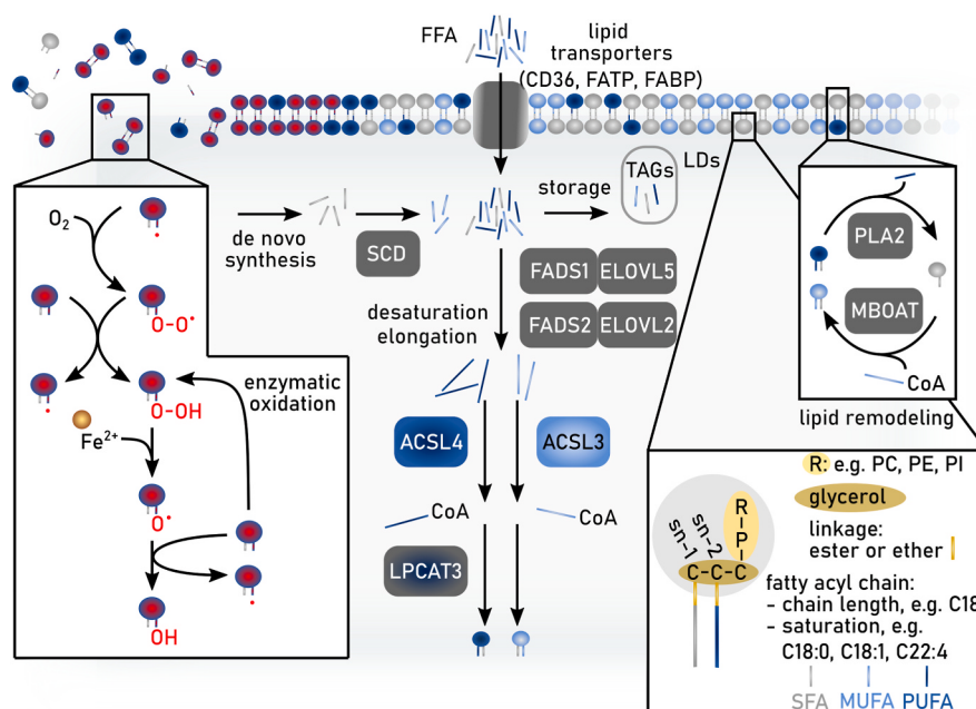
Fig. 4. Lipid metabolism and ferroptosis. Schematic overview of the main pathways involved in fatty acid biosynthesis and uptake, lipid synthesis and lipid remodeling that regulate ferroptosis sensitivity in cells. In general, two fatty acyl chains are linked to a glycerol backbone via an ester or ether bond. The fatty acids at the sn-1 position are generally saturated fatty acids (SFAs) or mono-unsaturated fatty acids (MUFAs), whereas the fatty acids at the sn-2 position can be SFAs, MUFAs or poly-unsaturated (PUFAs). Lipids attached to the glycerol can be e.g. phosphatidylcholine (PC), phosphatidylethanolamine (PE), or phosphatidylinositol (PI). Free fatty acids (FFA) from the microenvironment can be taken up via CD36, fatty acid transport proteins (FATP) or fatty acid-binding proteins (FABP). The intracellular pool of fatty acids is comprised of SFA as product of de novo fatty acid synthesis or uptake, together with either MUFAs or PUFAs as products of fatty acid desaturation and elongation. Noteworthy, certain PUFAs are essential and thus have to be taken up by aforementioned extracellular space. Depending on substrate specificity, fatty acids are desaturated by stearoyl-CoA desaturase (SCD) and fatty acid desaturases (FADS1 or FADS2). Further, different elongases e.g. ELOVL2 or ELOVL5 are synthesizing fatty acids (SFA, MUFA or PUFA) with longer carbon chains. Members of the acyl-CoA synthetase long chain family of proteins (e.g. ACSL3 or ACSL4) convert free long-chain fatty acids into fatty acyl-CoA esters that then can be utilized to become incorporated into membrane phospholipids (PL) mediated by e.g. lysophosphatidylcholine acyltransferase LPCAT3. Additionally, intracellular fatty acids can be stored into lipid droplets (LDs) as they are converted into triacylglyceride. Existing membrane phospholipids can be remodeled via the Lands Cycle. Here, hydrolysis of the fatty acid (e.g. PUFA) at the sn-2 position by PLA2 produces a lyso-PL and a following re-esterification of another fatty acid-CoA (e.g. MUFA) mediated by MBOAT1 leads to the remodeled membrane PL.
