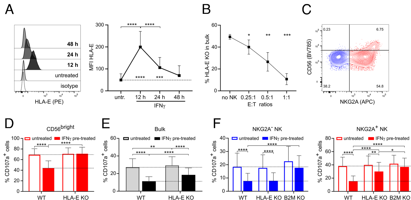
Figure 2 IFN \gamma -induced expression of HLA-E on A375 cells inhibits NKG2A + NK cells. (A) Expression of HLA-E on A375 cells treated or not with IFN \gamma for 12, 24 and 48 hours (n=6). (B) Reduction in HLA-E KO cell population after 24 hours of co-culture of NK cells with mixed WT:HLA-E KO cells (1:1) at different E:T ratios (n=6). (C) Representative dot plot showing the expression of NKG2A and CD56 on NK cells. (D, E) Degranulation of CD56 bright (D) and bulk NK cells (E) after 4 hours of co-culture with HLA-E KO or WT A375 cells. A375 cells were pretreated or not o/n with IFN \gamma (n=11). (F) Degranulation of NKG2A - and NKG2A + NK cells after 4 hours of co-culture with WT, HLA-E KO and B2M KO A375 cells pretreated or not with IFN \gamma 12 hours before the co-culture (n=6–9). Statistical analysis was performed by one-way ANOVA (multiple comparisons) test (A, B, D, E, F), *p<0.05, **p<0.01, ***p<0.001, ****p<0.0001. ANOVA, analysis of variance; E:T, effector to target; KO, knockout; NK, natural killer; WT, wild-type.
