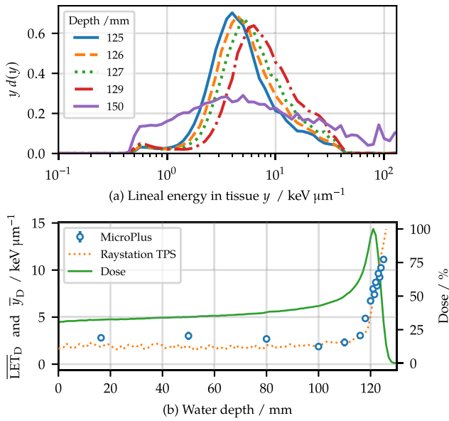
Fig. 17. (a) Microdosimetric spectra measured with the MicroPlus detector at different depths in a water phantom along 131 MeV proton spot scanning beam. (b) Determination of y_D to water with the MicroPlus detector along the central axis of a proton beam. The simulated \overline{\text{LET}}_D and dose with the Raystation treatment planning system is shown for comparison.
