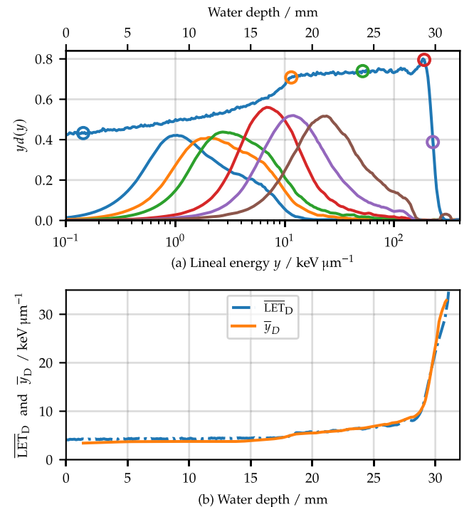
Fig. 15. (a) Microdosimetric spectra measured at six positions (indicated by open circles) in a 60 MeV proton spread-out Bragg peak (SOBP). The relative depth dose distribution is plotted for reference, where the marker color of the circles refer to the positions of the spectra. (b) Measured mean-dose lineal energy ( \bar{y}_D ) and simulated dose-averaged LET ( \overline{\text{LET}}_D ) along the central beam axis of the SOBP outlined in (a). Source: Data from Conte et al. (2019) and Bianchi et al. (2021).
