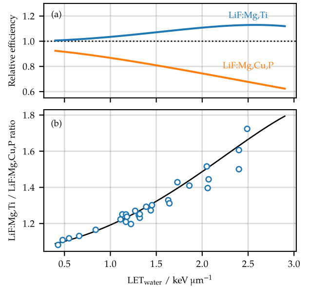
Fig. 6. (a) Relative efficiencies of LiF:Mg,Ti and LiF:Mg,Cu,P as calculated in Olko and Bilski (2021). (b) shows the ratio of the two functions in (a) plotted as a solid line against measurements (markers) acquired in proton beams. Source: Data from Sadel et al. (2015).
