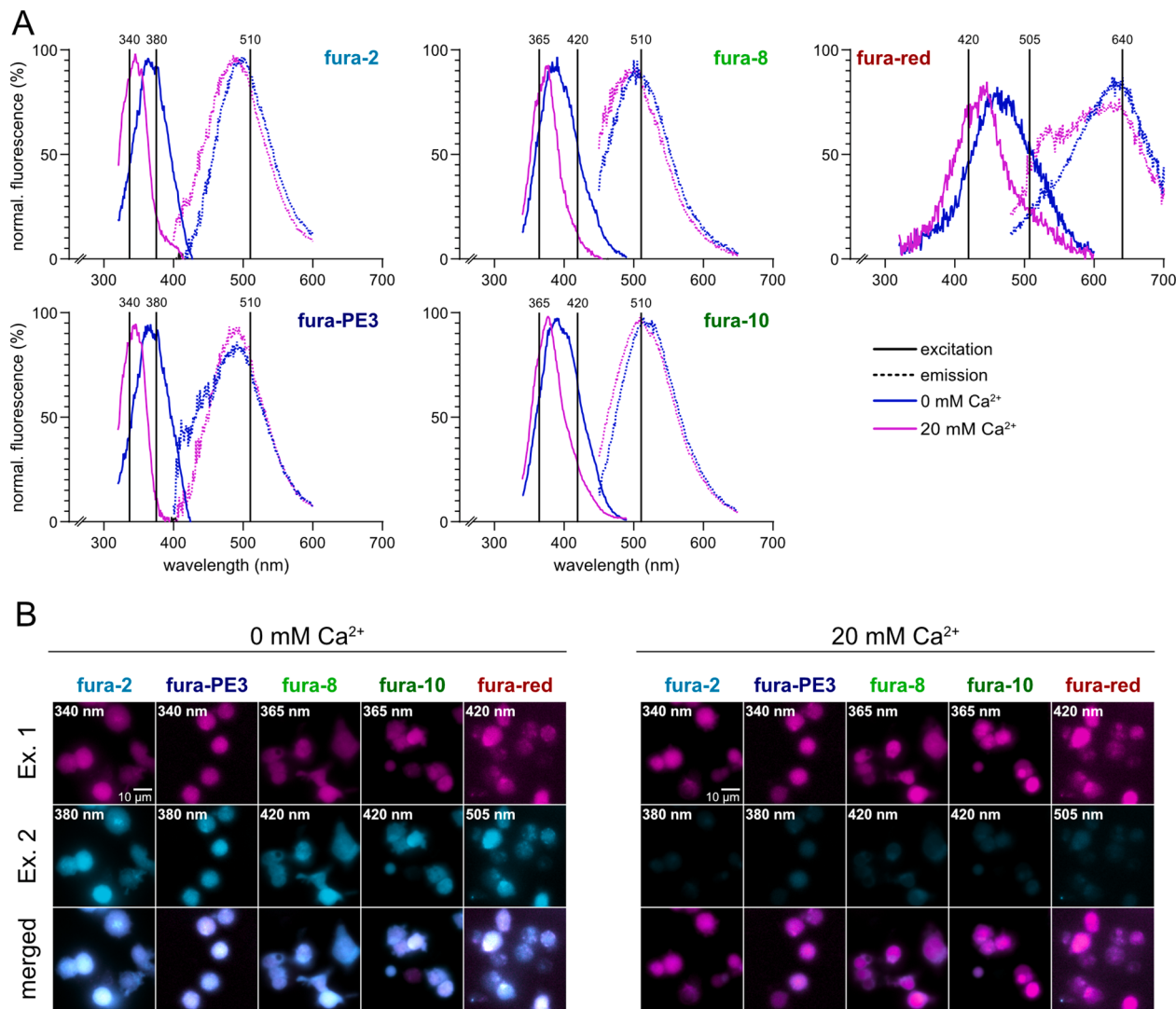
Fig. 1. Spectral properties and indicator loading in primary NK cells. (A) Excitation spectra for Ca 2+ bound and Ca 2+ free state (solid lines) and emission (dotted lines) spectra of fura-2-, fura-PE3-, fura-8-, fura-10-, and fura-red-loaded primary NK cells under low-Ca 2+ (0 mM Ca 2+ , 1 mM EGTA, blue) or high-Ca 2+ (20 mM Ca 2+ , magenta) conditions. Thapsigargin (1 μM) and ionomycin (4 μM) were added to both solutions. Spectra were recorded at 37 °C/5 % CO 2 in the plate reader. Data represent the mean of 5–15 measurements per condition. Vertical bars indicate the excitation and emission wavelengths used in subsequent experiments. (B) Representative images with the Cell Observer (40x) of primary NK cells loaded with each indicator, showing both excitation channels and the corresponding merged images for 0 mM Ca 2+ and 20 mM Ca 2+ conditions. Scale bar: 10 μm.
