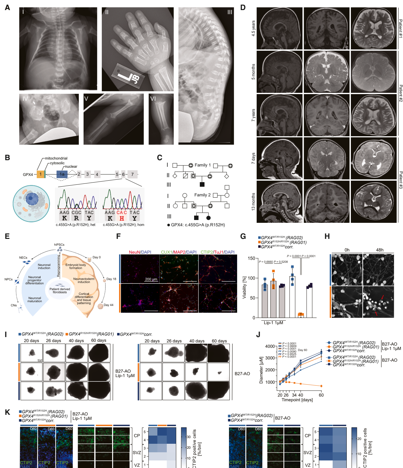
Figure 1. The GPX4 R152H allele triggers ferroptosis
