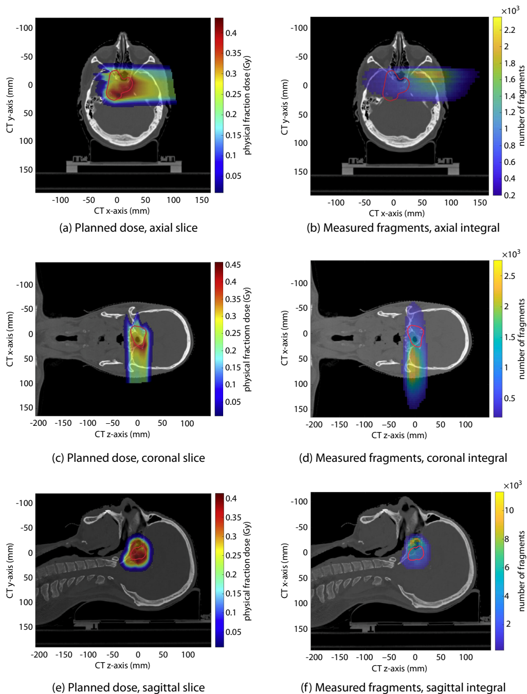
Fig. 2. (a, c, e) Slices of the planned physical dose distribution. (b, d, f) Integral fragment distributions measured with the monitoring system (treatment fraction 18). The red line delineates the planning target volume. Abbreviation: CT = computed tomography.
