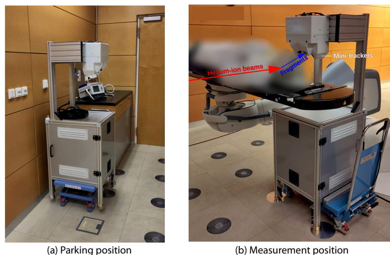
Fig. 1. (a) Photograph of the monitoring system in the parking position in the corner of the treatment room before and after therapy. (b) Monitoring system in the measurement position with the anonymized patient on the patient table.
