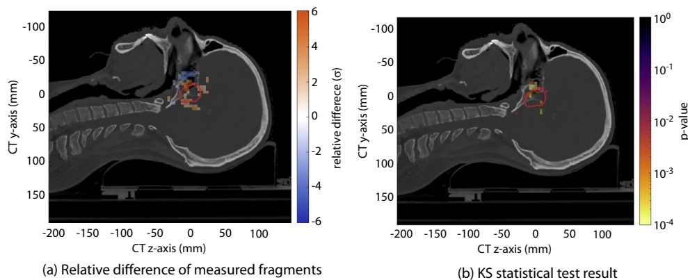
Fig. 3. Comparison of the measured fragment distributions in the sagittal plane. The red line delineates the planning target volume. (a) Relative difference of the measured fragment distributions. (b) Two-sample KS statistical test result of the measured fragment distributions. Abbreviation: CT = computed tomography; KS = Kolmogorov-Smirnov.
