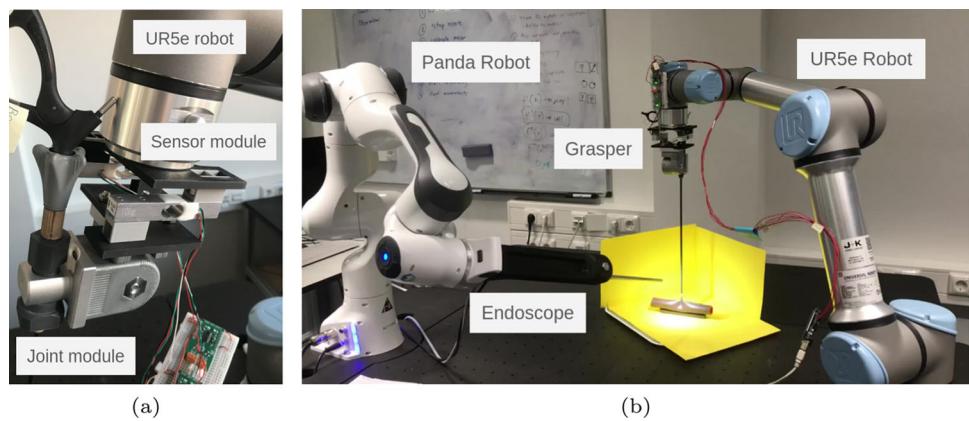
Fig. 1 Experimental setup in detail. a Mechanical design of the sensor module and the grasper joint. b Full setup with background and a phantom
