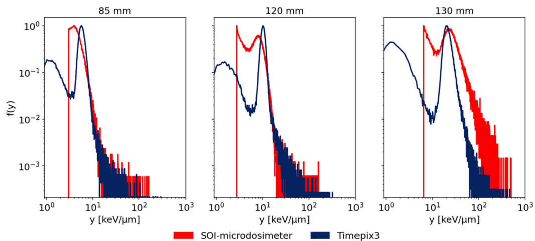
FIGURE 6 f(y) vs. y distribution in the log-log representation at different PMMA depths along the Bragg curve. The spectra are reported without material conversion i.e., silicon with density 2.33 \text{ g cm}^{-3} .
