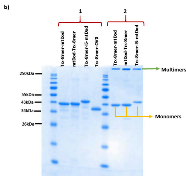
Fig. 1. Production of Trx-8mer antigens as fusion to mtDod. (a) Design of mtDod antigens as a fusion of the Trx-8mer with mtDod. mtDod: dodecin protein from Mycobacterium tuberculosis that forms dodecameric multimers, L2 20-38 8mer: the combination of L2 20-38 epitopes from eight different HPV types (16–18–31–33–35–6–51–59), that were selected based on sequence homology to the major cross-neutralization HPV16 L2 20-38 epitope. The 8mer polytope was inserted into the active center of the Trx scaffold to generate the Trx-8mer. A rigid proline-alanine-serine (PAS) linker connects mtDod to the rest of the protein. (b) SDS-PAGE analysis comparing the purity of mtDod antigens with Trx-8mer-OVX (PANHPVAX), used as a reference antigen for immunization. To completely disassemble the multimeric mtDod antigens, samples (1) were treated using a two-step sample preparation protocol. A mixture of monomeric and multimeric mtDod proteins (2) were obtained when samples were treated with a single-step protocol.
