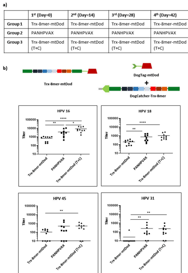
Fig. 8. Decoration of mtDod nanoparticles with Trx-8mer via DogTag/DogCatcher enables improved immunogenicity of the Trx-8mer antigen. (a) Trx-8mer-mtDod (T + C) represents the antigen mtDod decorated with Trx-8mer after assembly. (b) Sera from immunized mice ( n = 10 mice per group) were tested for neutralizing antibodies by using PBNA. Mice immunized with Trx-8mer-mtDod (T + C) exhibit significantly higher neutralizing antibody titers against all tested PsV types compared to those immunized with Trx-8mer-mtDod. 20 \mu\text{g}/\text{mouse} Trx-8mer-mtDod and PANHPVAX were injected, and Trx-L2 in Trx-8mer-mtDod (T + C) was adjusted to equimolar amounts in Trx-8mer-mtDod. The y-axis shows the serum neutralizing antibody titers as EC50 values. Each symbol represents the neutralizing antibody titer for one mouse. The horizontal lines indicate the means of the titers for each group. A p value of \leq 0.05 was considered significant. The p values are as follows: * < 0.05 , ** < 0.01 , *** < 0.001 , **** < 0.0001 . (c) To test whether DogTag/DogCatcher protein provides a boosting effect, anti-mtDod antibody titers were measured by using GST-mtDod-ELISA of the sera of Trx-8mer-mtDod-immunized mice versus Trx-8mer-mtDod (T + C) immunized mice. The EC50 value for each serum sample was calculated as the reciprocal of the serum dilution that results in half of the saturated signal. The Mann-Whitney test was performed using GraphPad and revealed no significant difference in antibody titers between the two groups.
