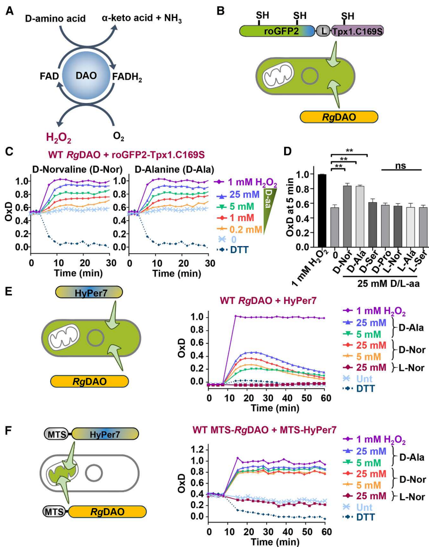
Figure 2. Initiating intracellular H_2O_2 fluxes by expression of D-amino acid oxidase from R. gracilis
